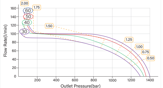
HFG-30/100-2 Pressure-Flow Rate Curves
