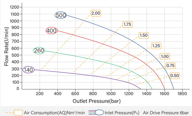
HFG-100D-2 Pressure-Flow Rate Curves
