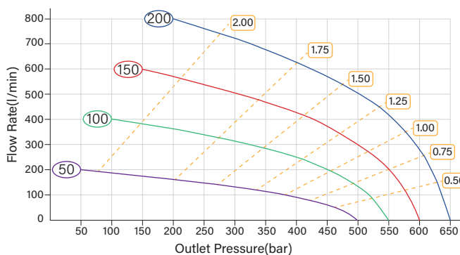
HFG-75D Pressure-Flow Rate Curves
