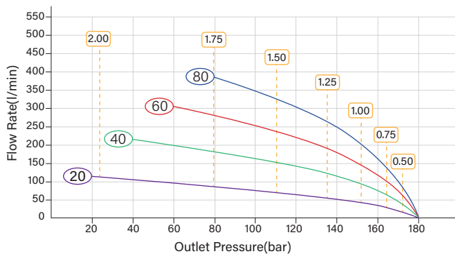
HFG-30 Pressure-Flow Rate Curves
