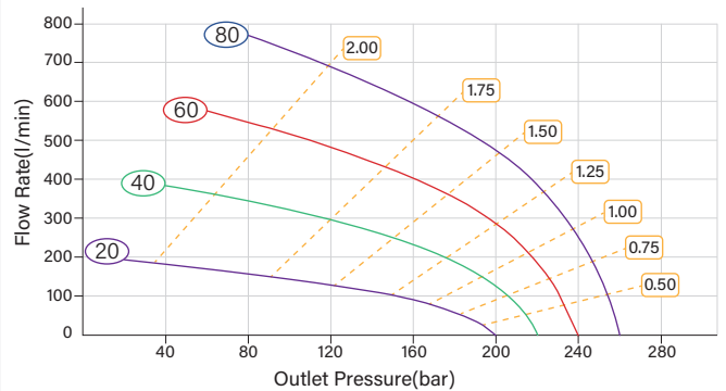
HFG-30D Pressure-Flow Rate Curves
