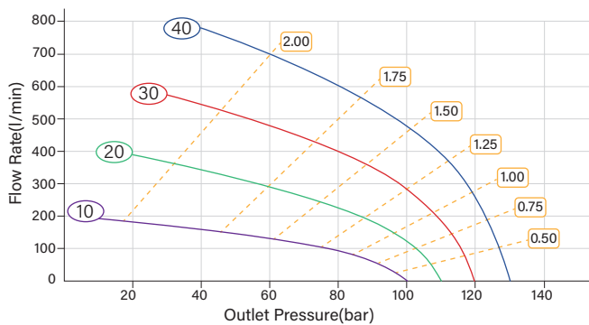
HFG-15D Pressure-Flow Rate Curves
