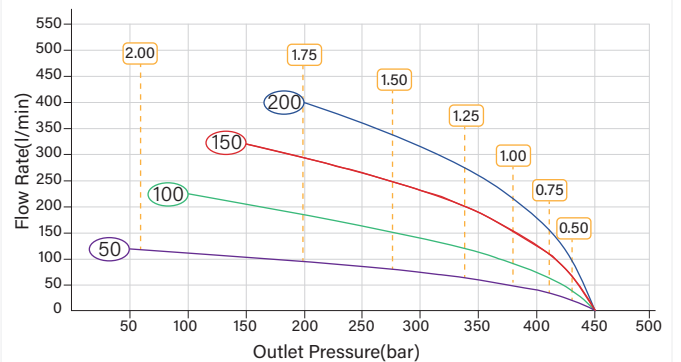
HFG-75 Pressure-Flow Rate Curves
