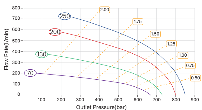
HFG-100D Pressure-Flow Rate Curves
