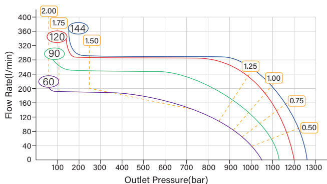
HFG-30/75-2 Pressure-Flow Rate Curves
