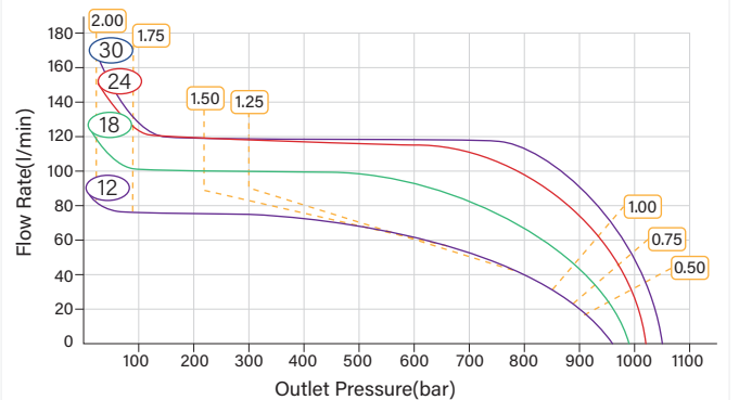
HFG-15/75-2 Pressure-Flow Rate Curves
