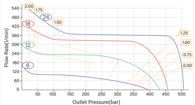
HFG-5/30-2 Pressure-Flow Rate Curves
