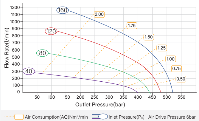
HFG-30D-2 Pressure-Flow Rate Curves
