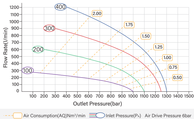
HFG-75D-2 Pressure-Flow Rate Curves
