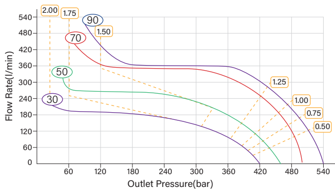
HFG-15/30-2 Pressure-Flow Rate Curves
