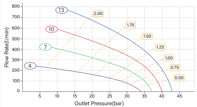
HFG-5D Pressure-Flow Rate Curves
