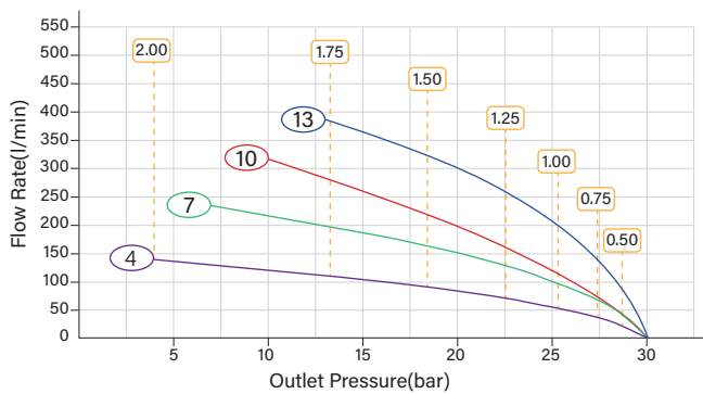
HFG-5 Pressure-Flow Rate Curves
