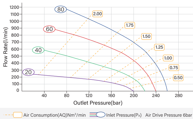
HFG-15D-2 Pressure-Flow Rate Curves
