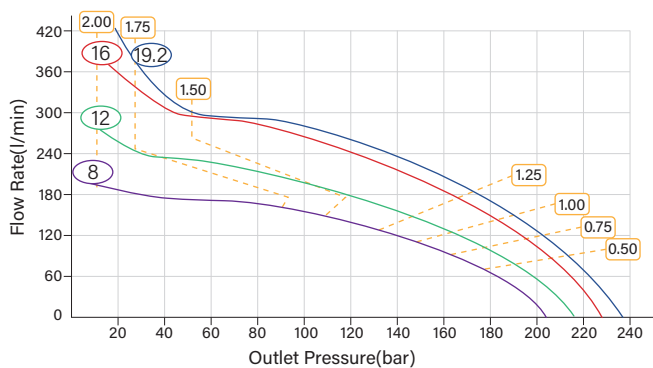
HFG-5/15-2 Pressure-Flow Rate Curves
