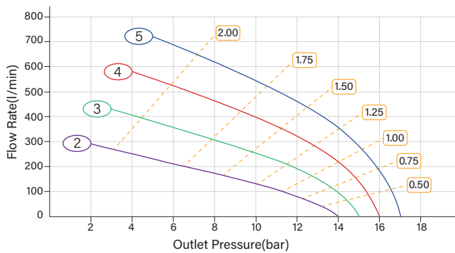
HFG-2D Pressure-Flow Rate Curves
