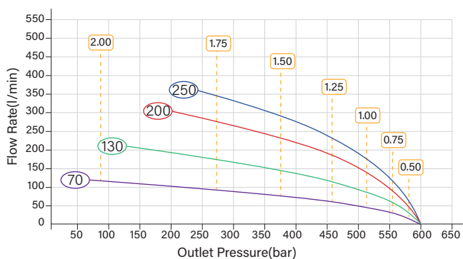
HFG-100 Pressure-Flow Rate Curves
