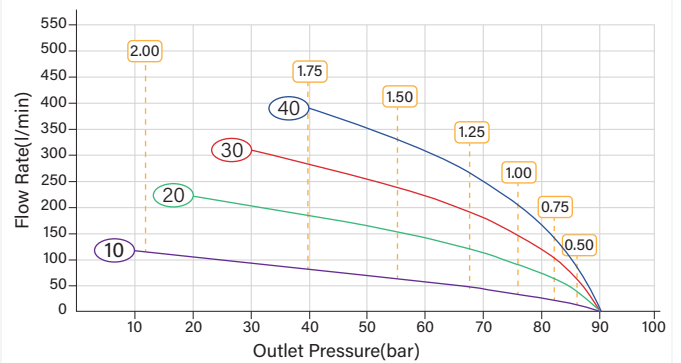
HFG-15 Pressure-Flow Rate Curves
