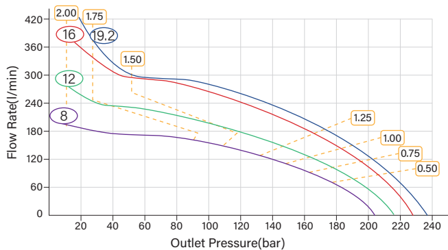
HFG-5/15-2 Pressure-Flow Rate Curves
