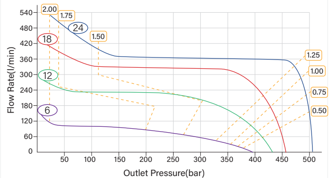
HFG-5/30-2 Pressure-Flow Rate Curves
