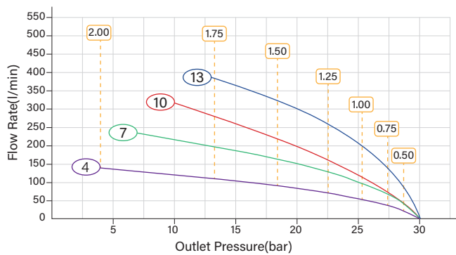
HFG-5 Pressure-Flow Rate Curves
