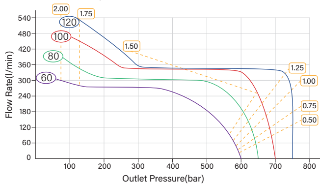
HFG-30/75 Pressure-Flow Rate Curves
