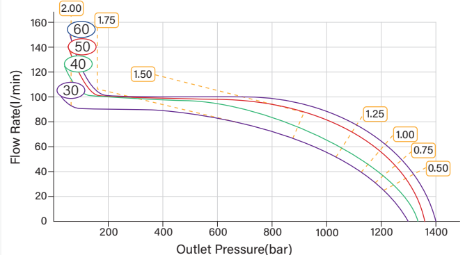
HFG-30/100-2 Pressure-Flow Rate Curves
