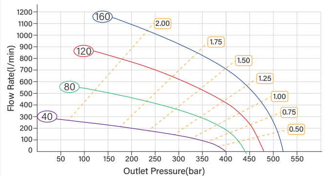
HFG-30D-2 Pressure-Flow Rate Curves
