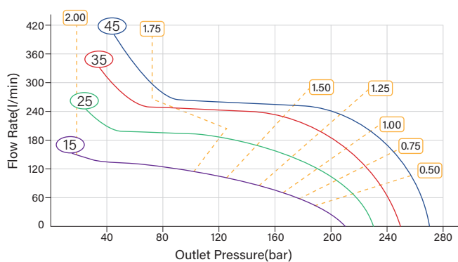
HFG-15/30 Pressure-Flow Rate Curves
