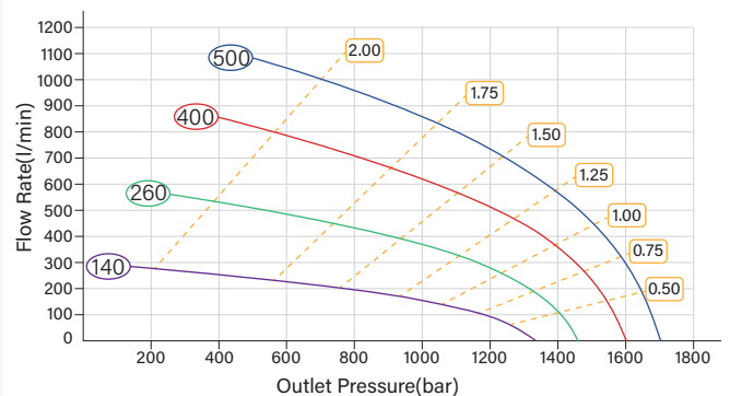
HFG-100D-2 Pressure-Flow Rate Curves
