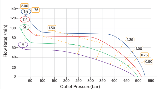
HFG-15/75 Pressure-Flow Rate Curves
