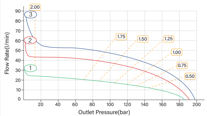
HFG-5/30 Pressure-Flow Rate Curves
