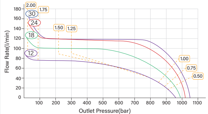
HFG-15/75-2 Pressure-Flow Rate Curves
