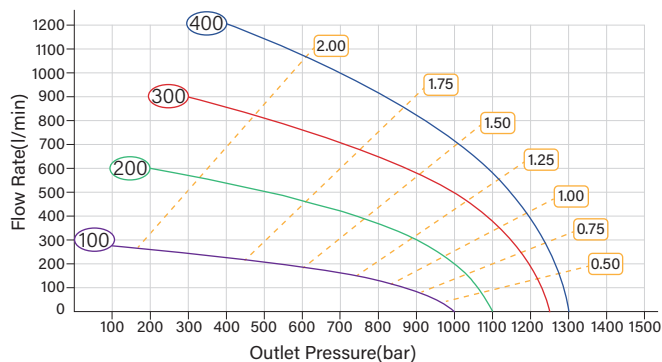
HFG-75D-2 Pressure-Flow Rate Curves
