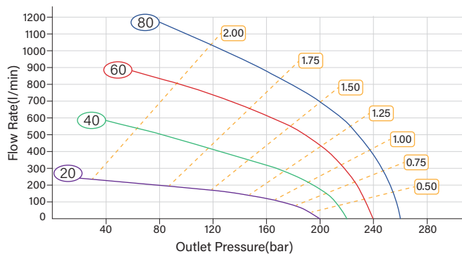
HFG-15D-2 Pressure-Flow Rate Curves
