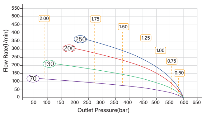
HFG-100 Pressure-Flow Rate Curves
