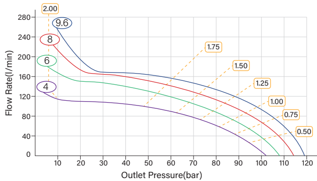
HFG-5/15 Pressure-Flow Rate Curves
