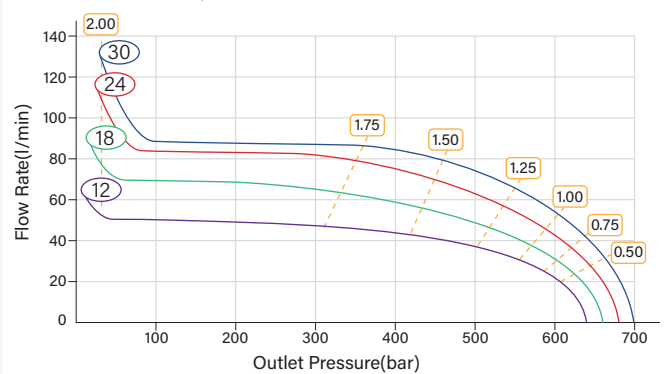
HFG-30/100 Pressure-Flow Rate Curves
