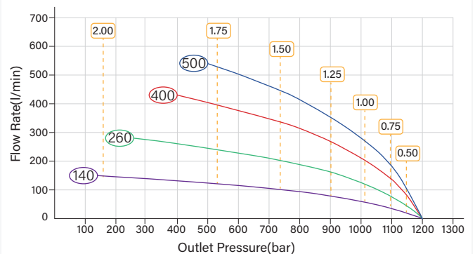
HFG-100-2 Pressure-Flow Rate Curves
