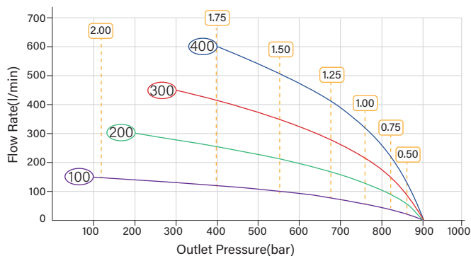
HFG-75-2 Pressure-Flow Rate Curves
