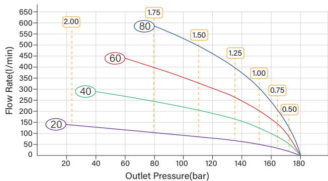
HFG-15-2 Pressure-Flow Rate Curves
