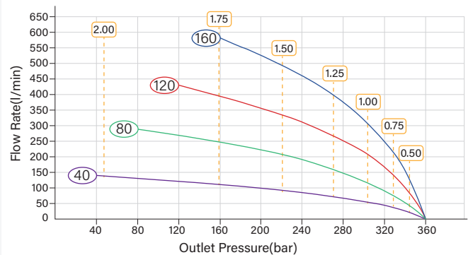
HFG-30-2 Pressure-Flow Rate Curves
